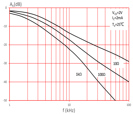
FIG.10: Frequency Response
