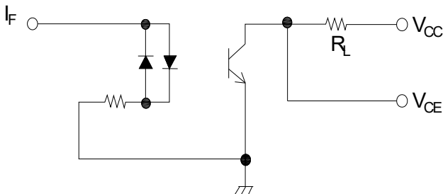
FIG.11: Test Circuits of Response Time
