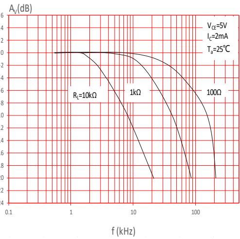
FIG.10: Frequency Response
