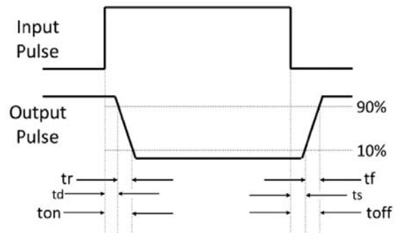
FIG.12: Curves of Response Time
