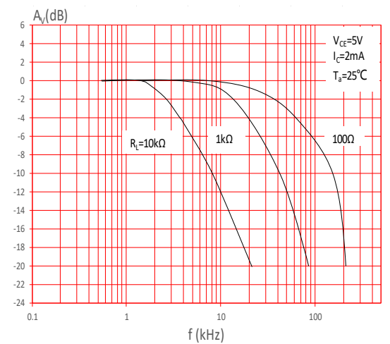
FIG.10: Frequency Response
